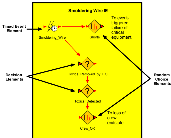
Fig. 6. Smoldering Wire Event Sequence Diagram Screen-shot from the GoldSim Model
