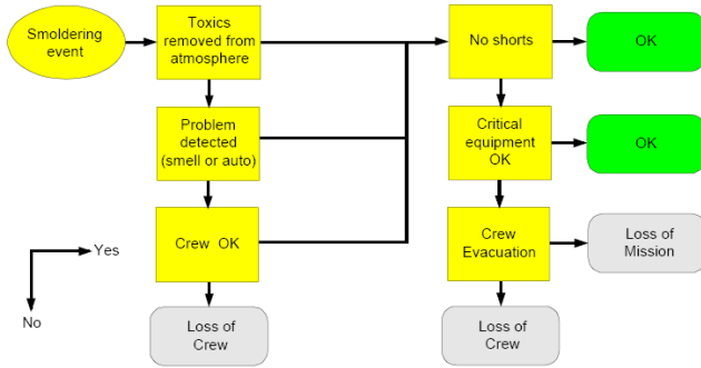
Fig. 5. Smoldering Wire Event Sequence Diagram [1]
