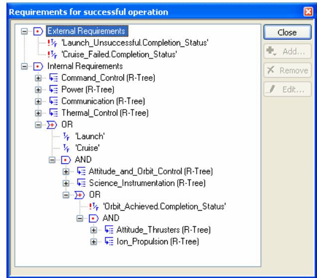
Fig. 8. Orbiter Requirements-tree Showing Dynamic Branch
