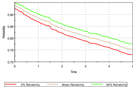
Fig.9. Orbiter Reliability over the Duration of the Simulation
