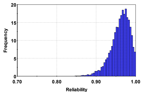
Fig. 10. Example of a Frequency Distribution of a Random (Aleatory) Process
