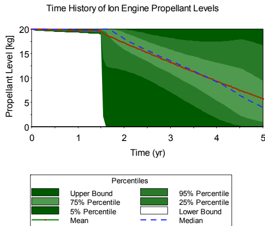
Fig. 13. Time History of Ion Engine Propellant Levels
