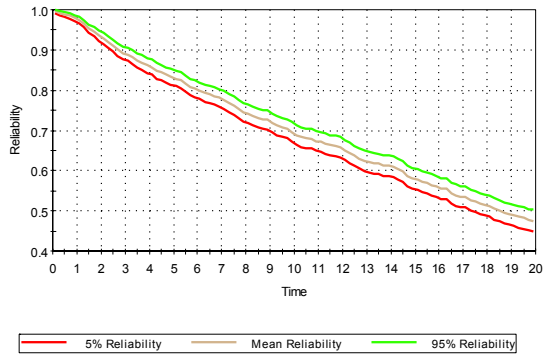
Fig. 7. Plot of Lunar Base Reliability Over the 20 Year Mission
