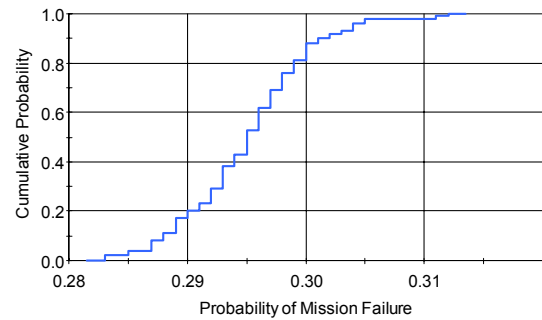
Fig. 11. Probability of Mission Loss From a Separated Uncertainty and Variability Analysis
