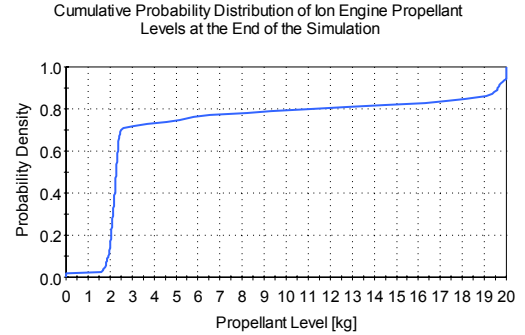
Fig. 14. Cumulative Probability Distribution of Ion Engine Propellant Remaining at the End of the Simulation
